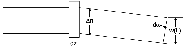
Figure 1. A thin atmospheric layer with varying index causes beam steering
