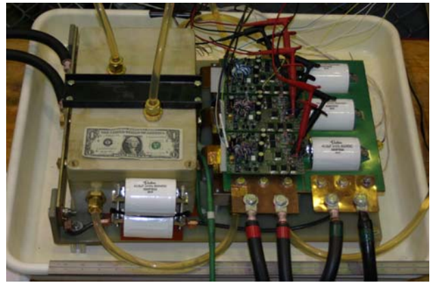
Fig. 1. ARL 90 kW bi-directional converter platform.
