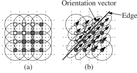
Fig. 1. Kernel spread in a uniformly sampled data set. (a) Kernels in the classic method depend only on the sample density. (b) Adaptive kernels elongate with respect to the edge.
