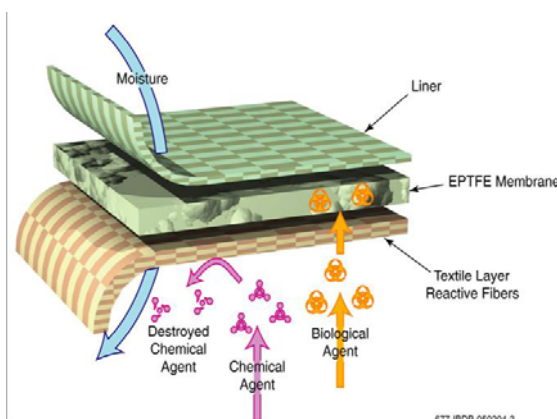
Figure 1: Nanocomposite multiplayer architecture (left) for self deactivation of chemical and biological threats. Cross section of the high surface area capillary-channeled (C-CP) fibers (right)
