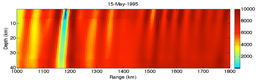
Figure 24: Range and depth at AAK for the May 15, 1995 Lop Nor test.
