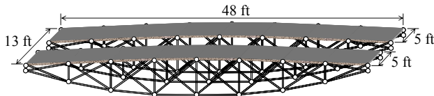
Fig. 2. Treadway System
