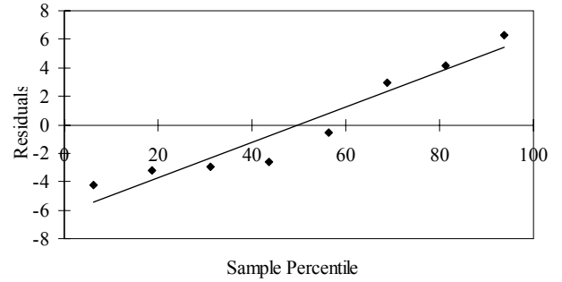
Fig. 13. Normal Plot of Residual Values
