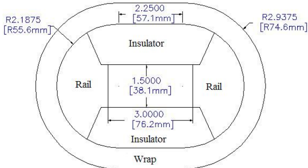
Fig. 1. Oval design
