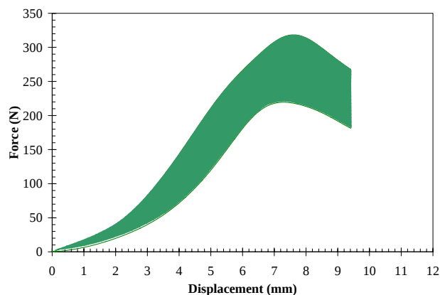
FIGURE 9: Force-deflection curve of human eye in-situ from blunt impact at 10 m/s. The synthetic eye and simulated extraocular fat in the FOCUS headform will match as closely as possible this force-deflection curve.
