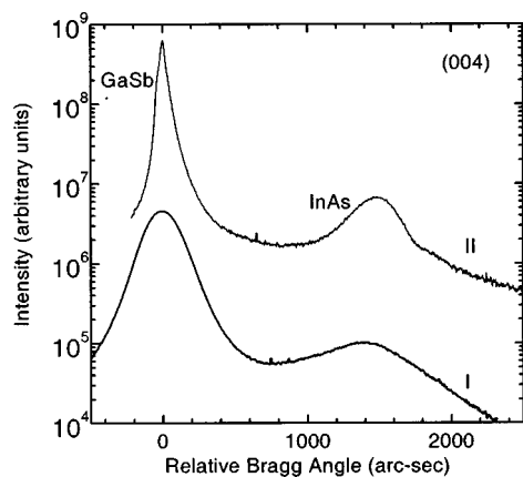
FIG. 2. Double-crystal x-ray diffraction data for two samples with 1000 Å InAs layers: (I) type-I structure with 4.0 \mu\text{m} GaSb buffer, (II) type-II structure.
