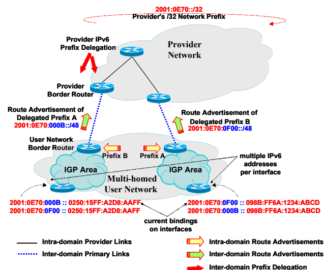
Figure 2: Multi-homed Battlefield Network
