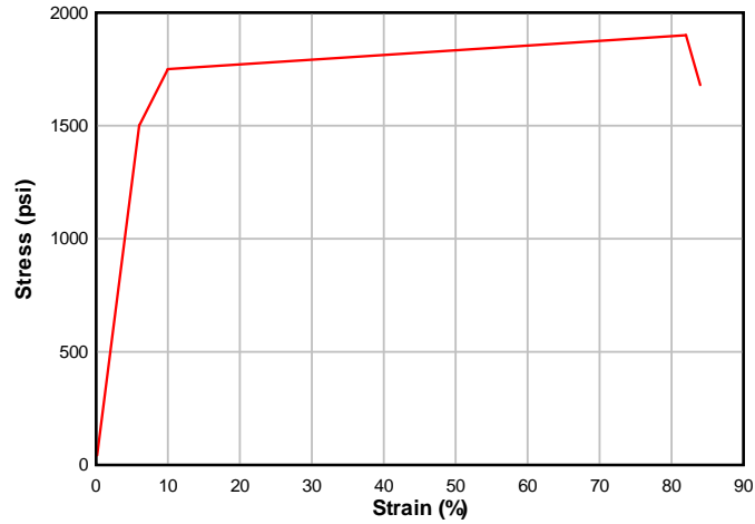
Fig. 3.1-4: Static stress-strain curve for the spray-on polymer
