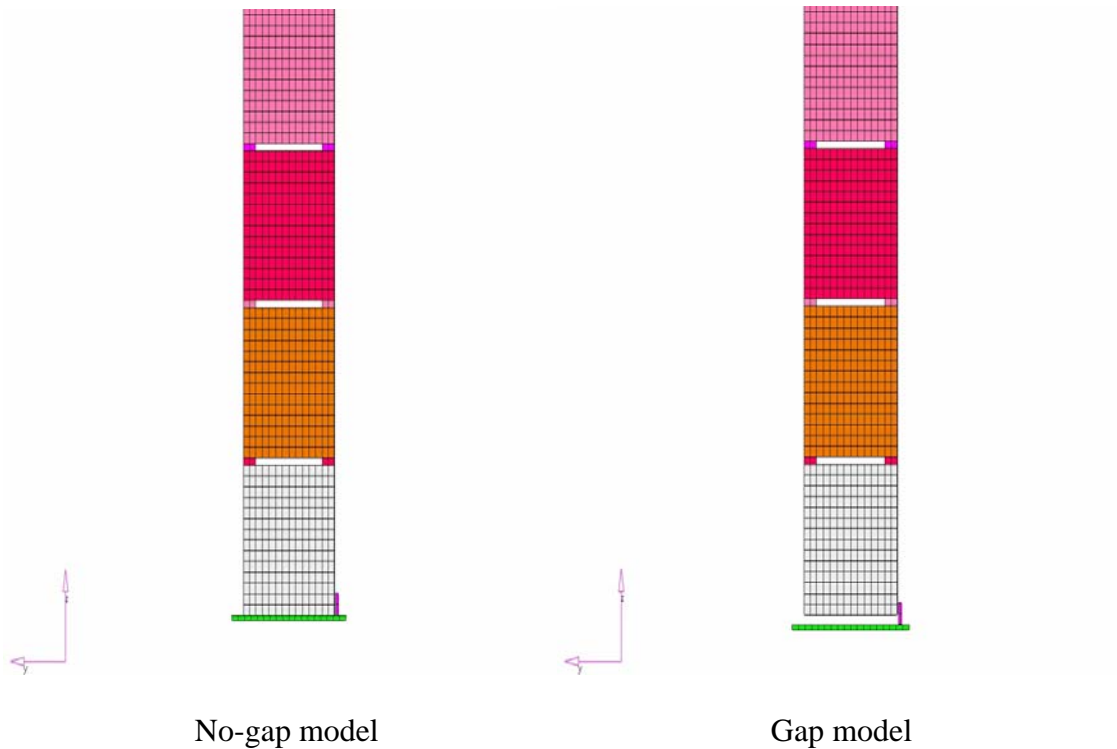
Fig. 7.1-1: F.E. model with and without gap
