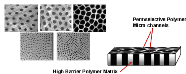
Figure 1 – Schematic of composite membrane (right) and various micrographs of actual microporous membranes (left).
