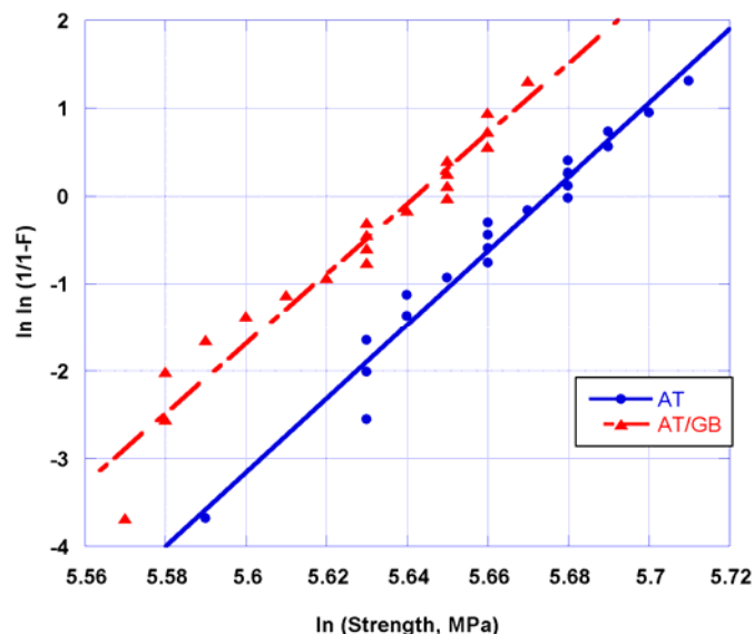
Figure 8. Weibull distribution for flexural strength of as-machined alumina subject to: 1) an acetone rinse (AT) and 2) an acetone rinse and grit blast.
