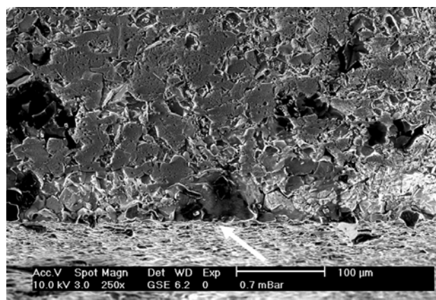
Figure 9. ESEM micrograph depicting the strength-limiting flaw in an AT alumina flexure specimen. The flaw, indicated by the white arrow is a sub-surface semi-elliptical crack induced by surface machining damage.
