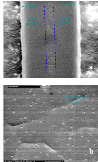
Fig. 8. Etch pit distribution in the (a) PE-GaN stripe in 2 \times 20 \mu\text{m} pattern and (b) conventional GaN layer grown simultaneously at the near vicinity of the striped PE-GaN. The bar in the SEM image is 4 \mu\text{m} .
