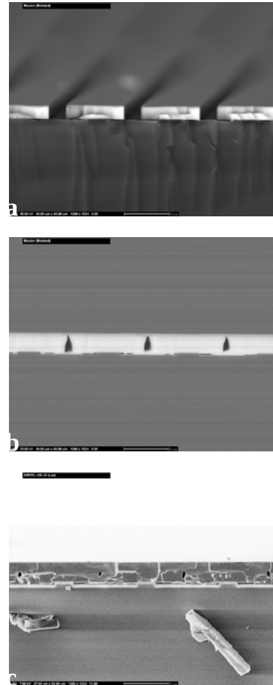
Fig. 6. PE-GaN growth progression in a 3 \times 14 \mu\text{m} pattern at (a) 30 min, (b) 60 min, and (c) 90 min and pressure of 100 Torr and V:III ratio of 2600.
