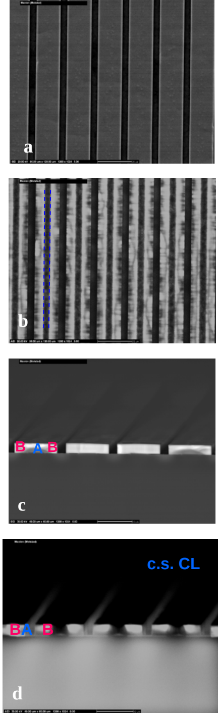
Fig. 10. SEM and the corresponding CL image in plan view (a, b) and cross-section (c, d) from PE-GaN structure in 2 \times 14 \mu\text{m} pattern. Note that in the CL images (b) and (d) the seed/column regions associated with high density of dislocations appear dark and in contrast, the regions of lateral PE-GaN growth appear bright.
