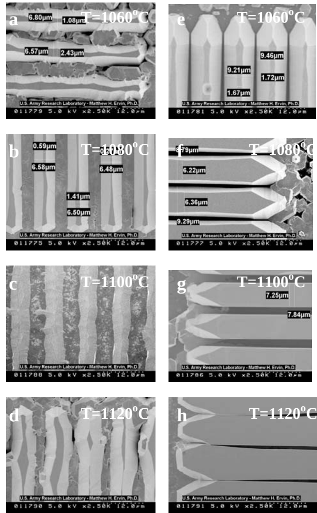
Fig. 3. Plan view SEM images of uncoalesced PE-GaN structures grown at different temperatures and crystallographic orientations of the stripes: along [11-20] (a-d) and along [1-100] (e-h).
