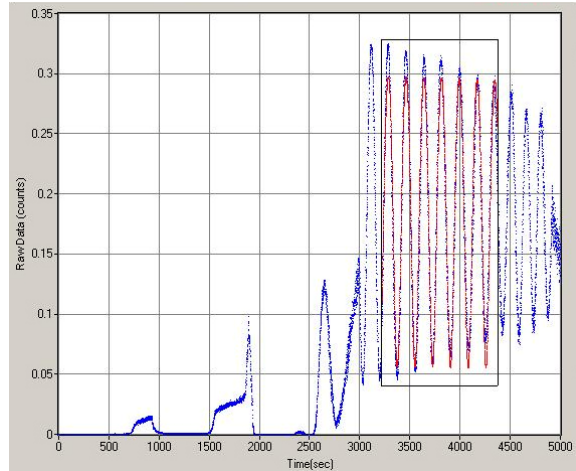
Fig. 2. Reflectance recorded during standard MOCVD growth of underlying seed GaN on (0001) sapphire substrate.
