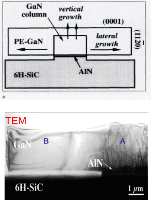
Fig. 1. (a) A schematic of the pendeo-epitaxial GaN approach. GaN grows vertically and laterally at the same time (b) Transmission electron microscopy (TEM) of pendeo-epitaxial GaN revealing two to four orders of magnitude lower density of dislocations in the regions of lateral growth (B) compared to the regions of vertical growth (A).
