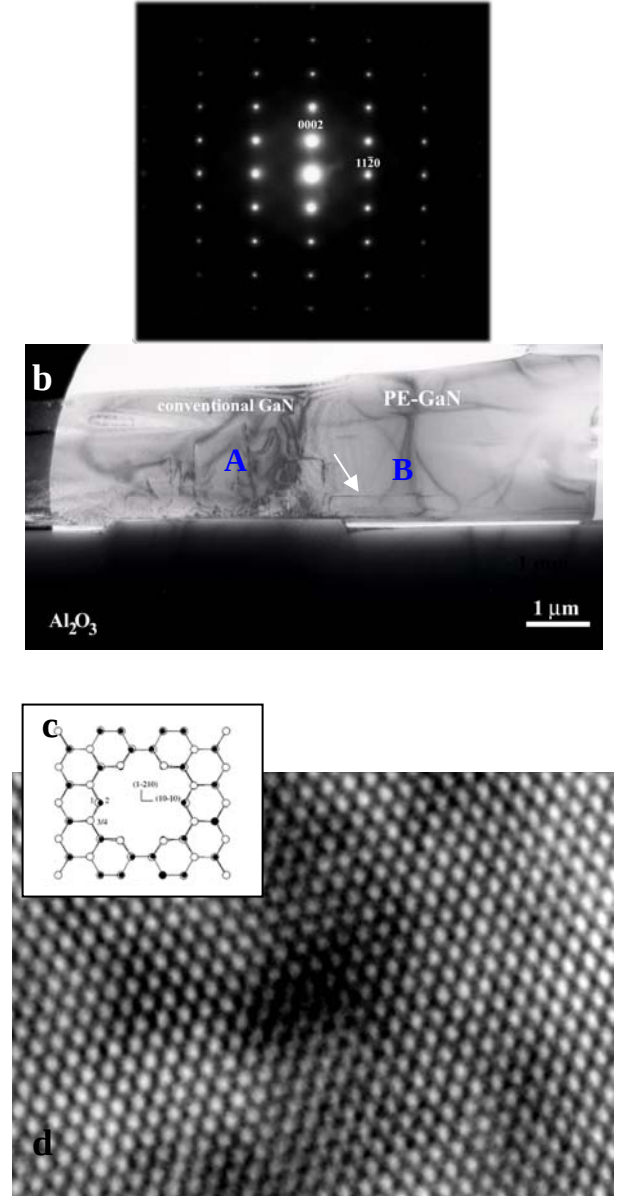
Fig. 9. (a) Selected area diffraction pattern, (b) cross-sectional TEM, (c) a schematic of an open core screw dislocation and (d) plan view HRTEM from an open core screw dislocation in PE-GaN heterostructure
