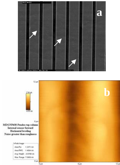
Fig. 7. (a) SEM image from the top (0001) surface of the PE-GaN stripes in 2 \times 14 \mu\text{m} pattern. (b) AFM micrograph acquired from the (0001) GaN stripe area.
