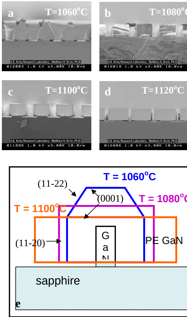
Fig. 4. Development of the top and side walls surface morphology and crystallography at different growth temperatures (a) 1060, (b) 1080, (c) 1100, and (d) 1120 ^{\circ}\text{C} . (e) A schematic of the side wall crystallography at different growth temperatures.
