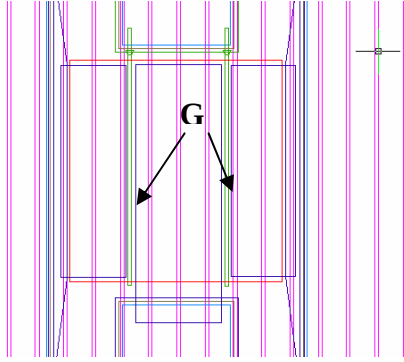
Fig. 11. PE-GaN HEMT mask designed to position the gates over the low defect density PE-GaN regions to test the device performance and reliability
