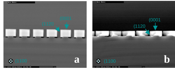
Fig. 5. Variation of the vertical to lateral growth rate ratios at two different V:III ratios: (a) 1040 and (b) 2600.
