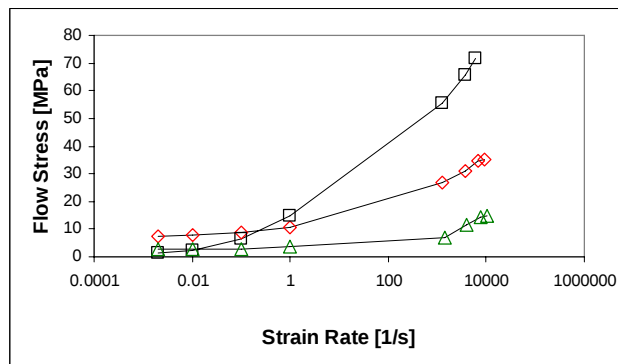
Fig. 6. Flow stress (taken at strain 0.15) vs strain rate data for BDO-containing PU's with 54 wt.% ( \diamond ) and 44 wt.% ( \triangle ) hard segment content, and for DMPD-containing PU with 55 wt.% ( \square ) hard segment content (Yi et al., 2006); flow stress values at 0.002 s^{-1} are 7.3 MPa, 2.6 MPa and 1.6 MPa for PU-B-54 ( \diamond ), PU-B-44 ( \triangle ) and PU-D-55 ( \square ), respectively, which were used for correlation with apparent crosslink density and fold recovery data.
