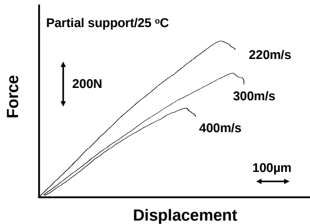
Figure 16: Typical force-versus-displacement curves in flexure determined from SiC/SiC target specimens impacted at three different velocities by 1.59-mm steel ball projectiles in partial support at ambient temperature (25°C). The peak of each curve indicates a fracture force.
