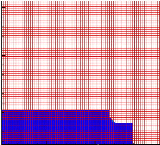
Figure 5. Discretized disk charge
