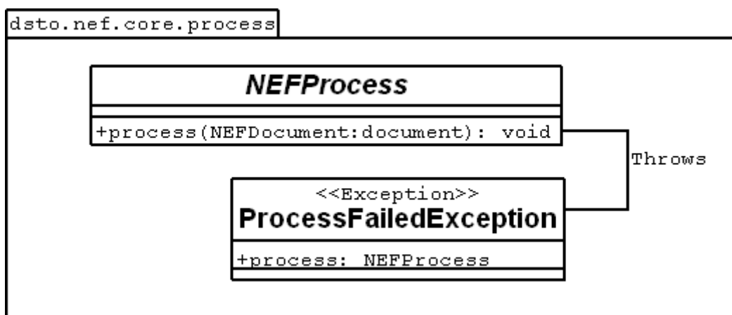
Figure 8 dsto.nef.core.process Package
