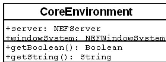
Figure 3 dsto.nef.core.CoreEnvironment
