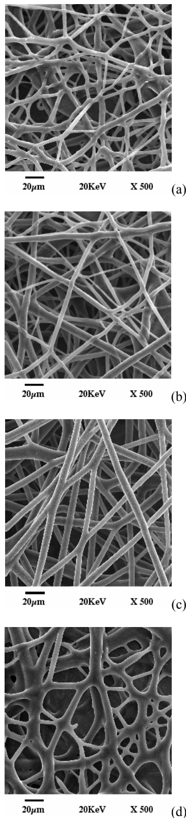
Figure 2. SEM of prepared butyl rubber membranes with two different carbon blacks at 25 phr: (a) N-134, (b) N-220, (c) N-550, and (d) N-990
