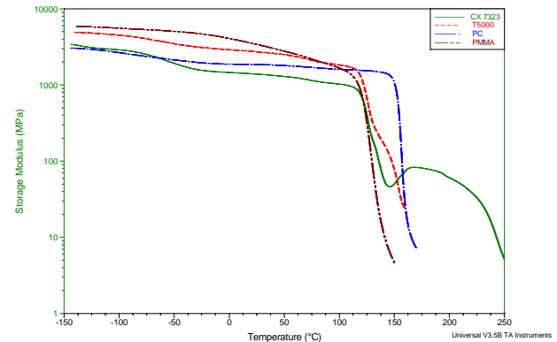
Figure 3. DMA scan of Flexural modulus ( E' ) as a function of temperature of PC, PMMA T-5000 and CX-7323
