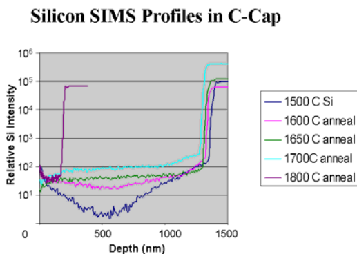
Figure 3: The apparent Si out-diffusion increases with the annealing temperature. Also, the cap for the 1800°C sample is much thinner. All graphs have been offset to allow for visual comparison.
