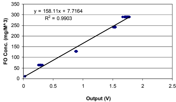
Figure 10. Linear regression calibration of RAS-4.
