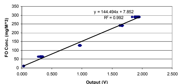
Figure 7. Linear regression calibration of RAS-1.
