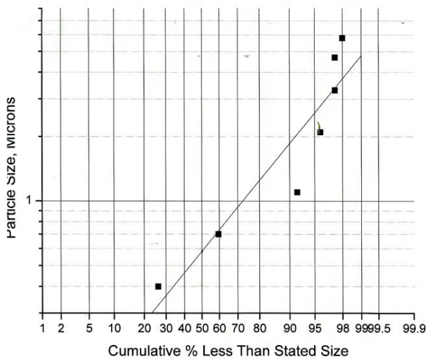
Figure 11. Anderson sampler plot of fog oil particle size distribution.
