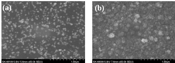
Fig. 7 SEM images of the as-deposited \text{TiO}_2 films (plan-view) on bare silicon substrates. Deposition conditions are (a) 8.8 mM \text{TiCl}_4 + 0.05 M HCl precursor solution, 70^\circ\text{C} , 4 h (2 steps, each 2 h). (b) 8.8 mM \text{TiCl}_4 + 0.05 M HCl precursor solution, 70^\circ\text{C} , 8 h (4 steps, each 2 h).
