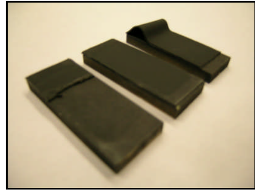
Figure #8 Control Specimens UDRI-R1, R2, R3 Rain Erosion Test
