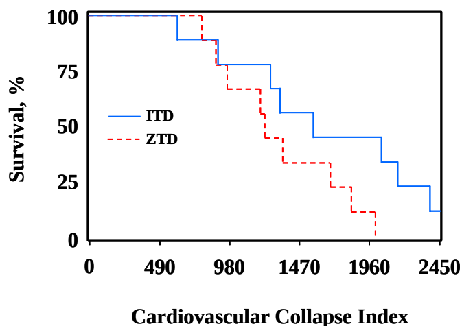
Fig. 7. LBNP completion (plotted as survival) curves of 9 subjects treated with an ITD (blue curve) and ZTD (red curve).
