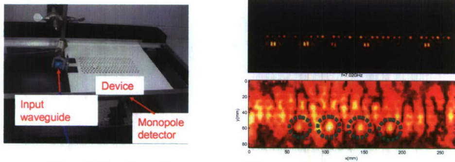
Figure 9. Experimental measurement of the tapping structure of the correlator
