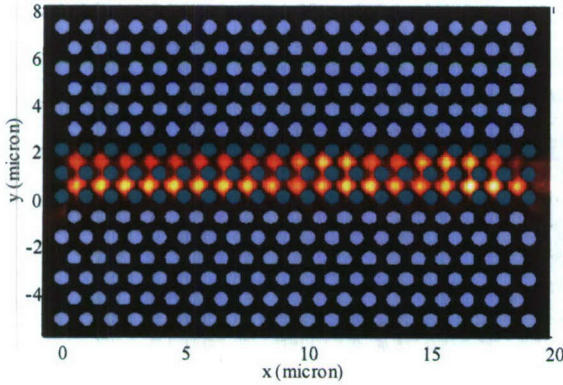
Figure 7. Hybrid lattice structure of photonic crystal
