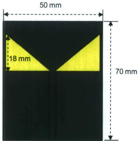
Figure 2. Bowtie antenna design for the correlator
