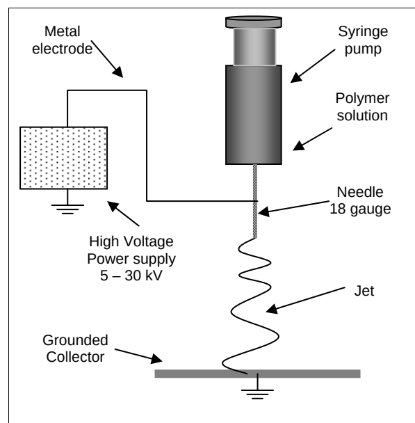
Fig. 2 Schematic of electrospinning process
