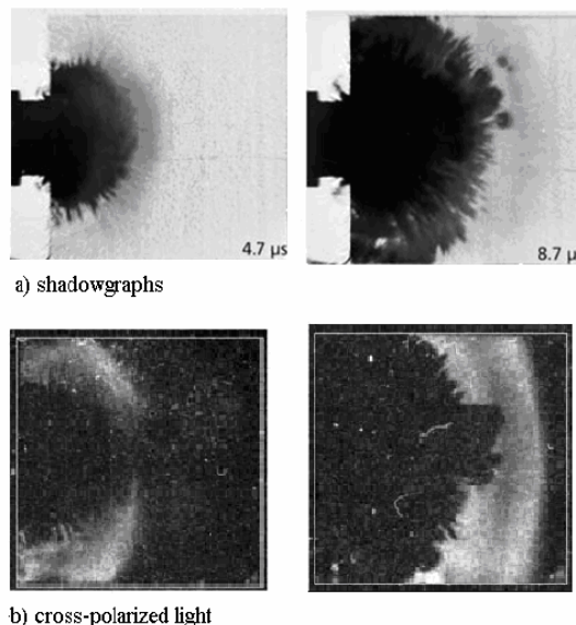
Figure 1. Selection of two shadowgraphs and corresponding crossed polarizers pictures from impact on AION at 380 m/s
