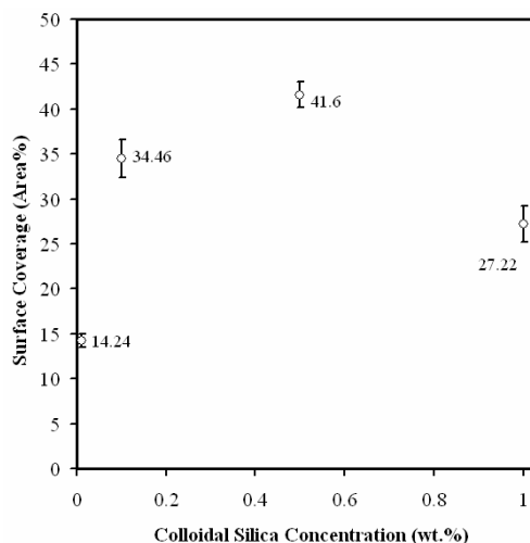
Fig. 11. Surface coverage of the surfaces given in Fig. 10 (calculated as described in Section 2.3).
