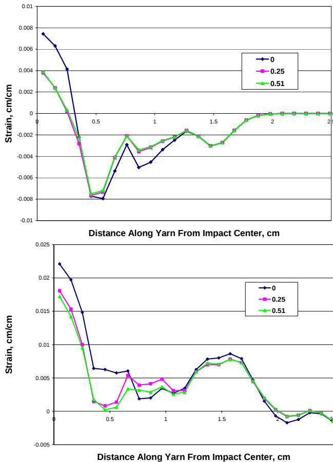
Figure 4. Strain distributions along impacted yarn for various friction coefficients at (top) 1.3 microseconds and (bottom) 2.8 microseconds.
