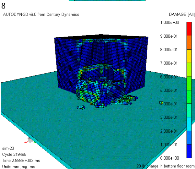
Fig. 7 SIM 20 20lb TNT Charge Within a Multi-Room Building. The frame sequence begins with 1 and progresses to 9 with sequence number noted at lower left.
