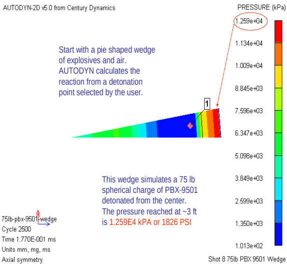
Fig. 2 Wedge Calculation
