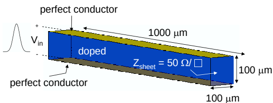
Fig. 4: A parallel conductor transmission line with a doped semiconductor serving as a lossy substrate and a 50 \Omega termination at the output.
