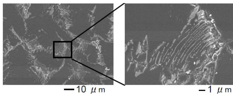
Fig. 3 SEM patterns of the part of the sample, which was exposed to a YAG laser ray. ( TiB_2:B_4C = 12:88 )
