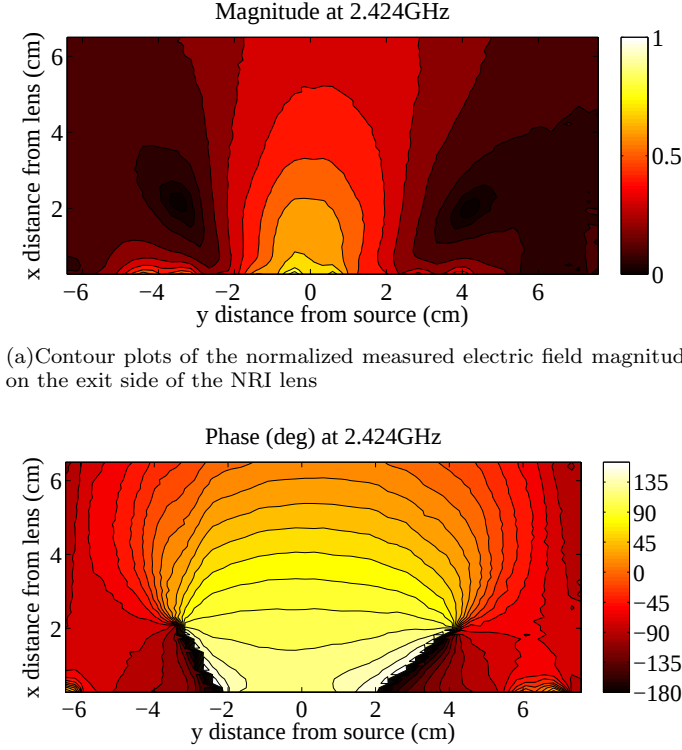
(b) Contour Plots of the Measured Unwrapped Electric Field Phase on the exit side of the NRI lens
