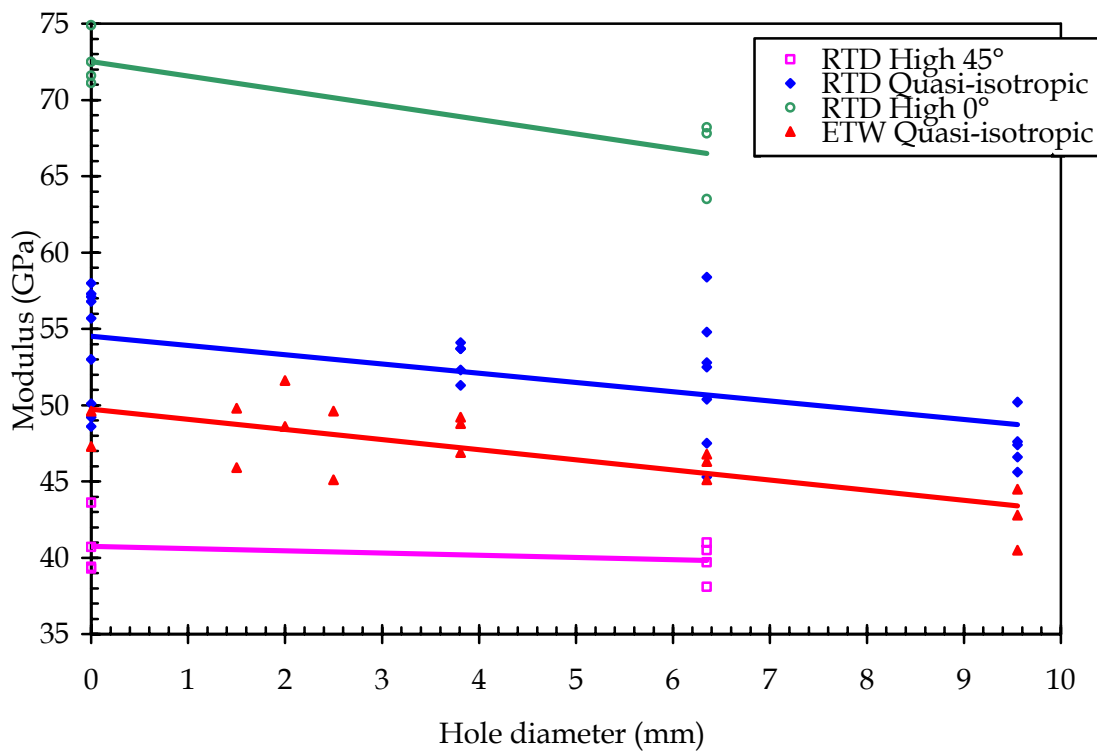
Figure 47: The effect of hole size on the modulus of OHB specimens
