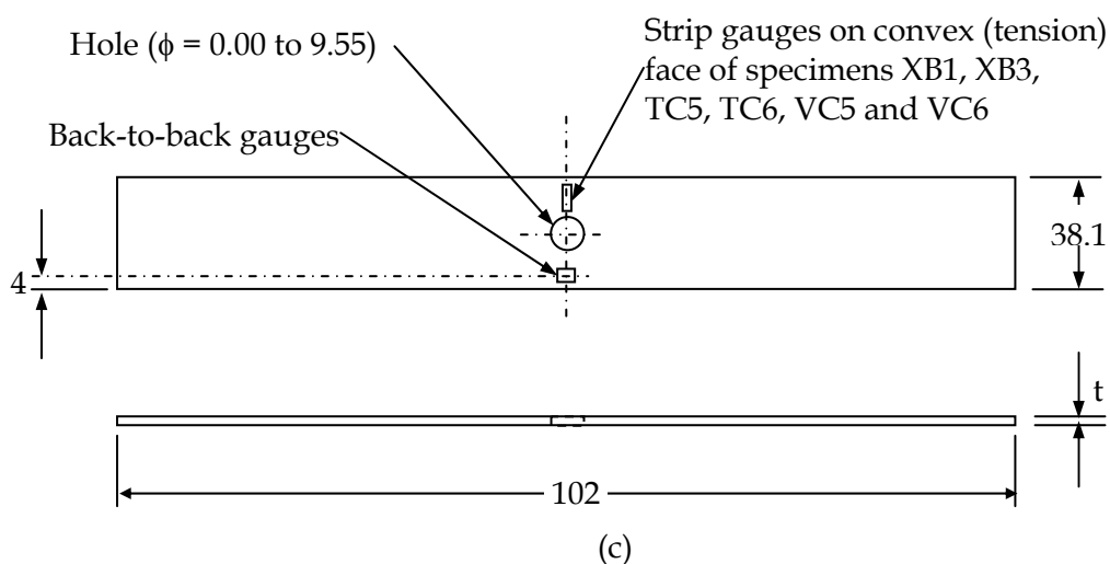
Figure 6: Diagrams of (a) OHT, (b) OHC and (c) OHB specimen showing dimensions in mm, strain gauge locations and extensometer locations
