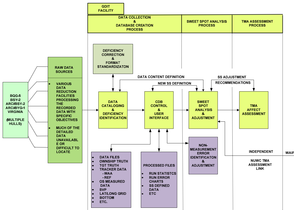
Figure 3. Overall Process Flow
