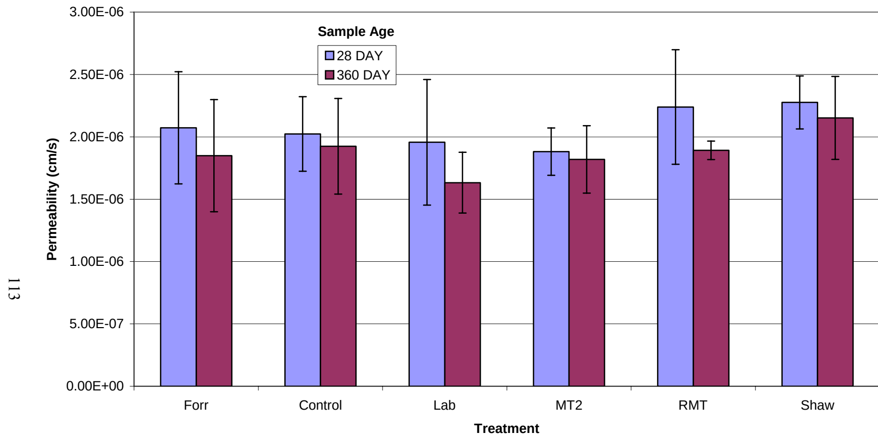
Figure 7-30. Permeability of the control and vendor-treated soils.
