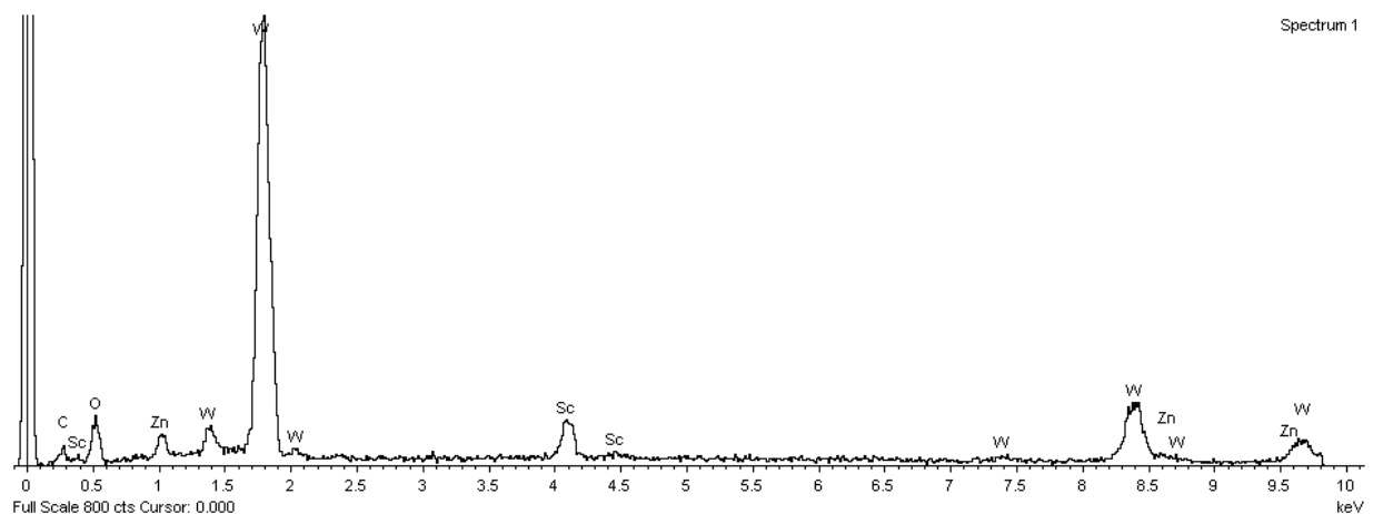
Figure 11. EDAX spectrum of surface regions indicated in Figure 10
