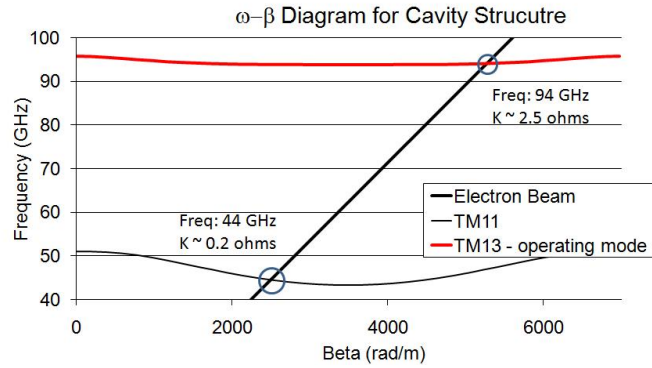
Figure 20. Dispersion diagram for the slow wave structure. The TM_{130} operating mode is shown in red. The lower frequency TM_{110} parasitic mode is shown in black. Also shown is the electron beam line for a 40 kV beam. The circuit is operated in the first forward space harmonic corresponding to 270 degrees phase advance between two adjacent cells.
