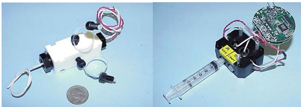
Figure 1. The spectrophotometric cell (left) and the dual channel fluorescence cell (right) form the optical core of the single channel nutrient analyzers under collaborative development.
