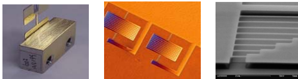
Figure 7. Successively smaller oscillators will enable devices capable of extremely high frequency sensing.
