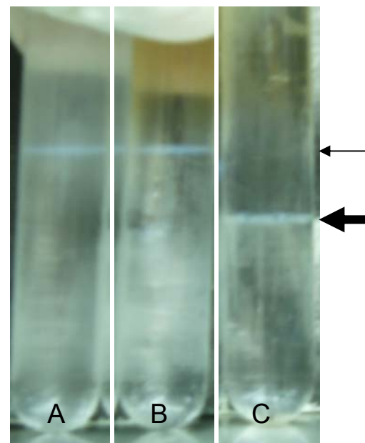
Fig. 2 Photographs of CsCl density gradient centrifugation of (A) Ad vectors alone, (B) Ad vectors without a 6-His tag but with Ni-NTA AuNP and (C) Ad vectors labeled with 6-His in hexon, coupled to Ni-NTA AuNP. Note the similar density of Ad bands in (A) and (B), indicating that no unspecific interaction occurs between Ad and AuNP (thin arrow). In contrast, Ad vectors labeled with 6-his in hexon clearly increased in density (C), indicating successful coupling of AuNP.
