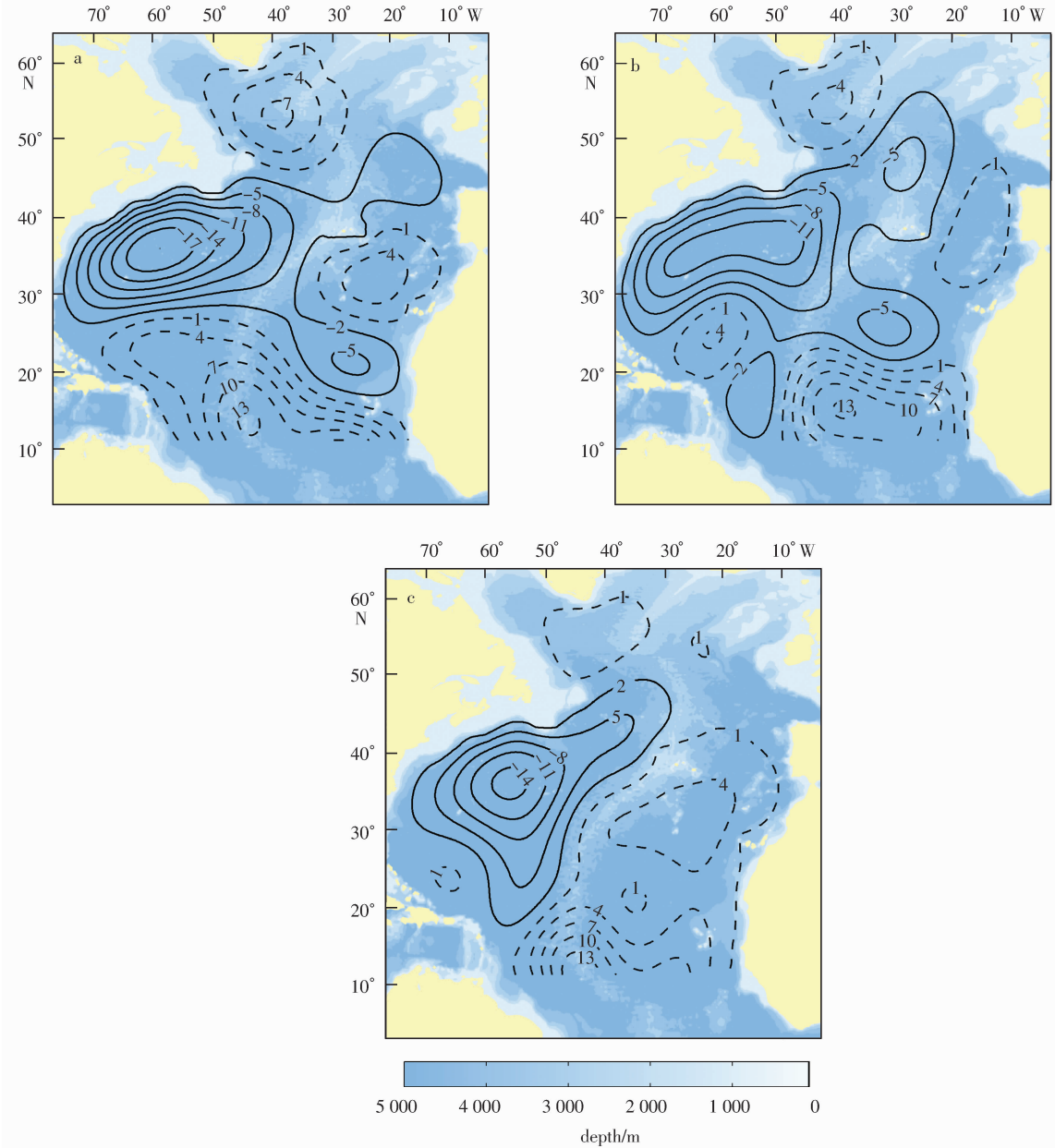
Fig. 4. Mean stream-function at 1000 m for December 2003—March 2004 (a) April 2004—July 2004 (b) and August 2004 November 2004 (c) computed by the OSD method. Contours are labeled in units of 10^7 \text{ cm}^2/\text{s} . The kinematic boundary and open boundary conditions used at \Gamma_1 and \Gamma_2 , and \Gamma_3 , respectively, are explained in Chu et al. (2003).
