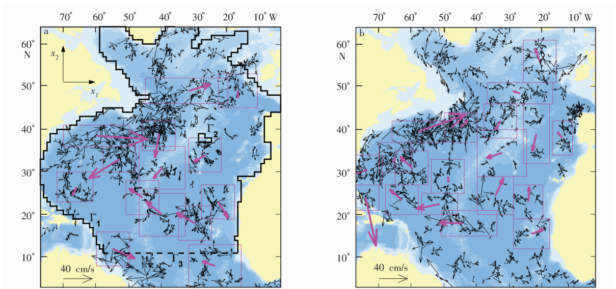
Fig. 1. Circulation velocities (tiny arrows) estimated from the original Argo float tracks at 1000 m for December 2003—Mar 2004 (a) and August 2004—November 2004 (b). The figure scale is given for tiny arrows. Red arrows are circulation velocities obtained by averaged over appropriate bins (red lines). The magnitudes of these arrows are multiplied by the scale equaled 20 for better visualization of schematic circulation patterns. \Gamma_1 , \Gamma_2 and \Gamma_3 are boundaries of the computation area.
