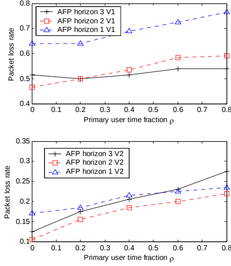
Fig. 12. Packet loss rate vs. time fraction \rho of the primary users occupying frequency channel F_1 around network node n = 7, 11, 12 (average T = 5.5\text{Mbps} , b_n / c = 1 , H_n^I = 80 meters).
