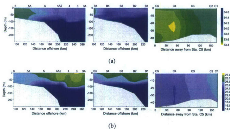
Fig. 8. Salinity (a) and temperature (b) distribution on Transect-A, B and C (from left to right) in November 2002.
