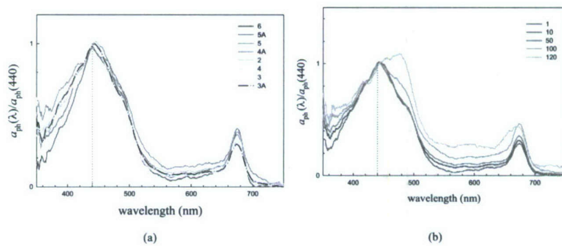
Fig. 10. \alpha_{ph} normalized at 440 nm in November 2002. (a) Surface distribution on Transect A; (b) Vertical distribution at Sta. 3. The legend in (b) shows the sampling depths in meters. The dotted vertical line in the graphs highlights the normal absorption peak at 440 nm.
