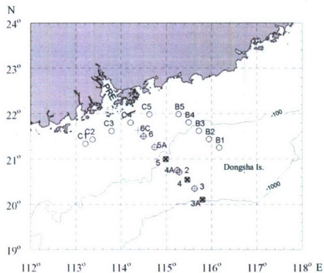
Fig. 1. CTD and sampling stations in the northern South China Sea. +: CTD and sampling stations in May 2001; x: stations only for CTD in May 2001; O: CTD and sampling stations in November 2002; PRE: the Pearl River Estuary; Dongsha Is.: Dongsha island.
