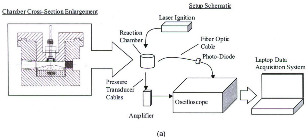
Figure 9 Constant volume reaction chamber includes pressure and light intensity measurements
