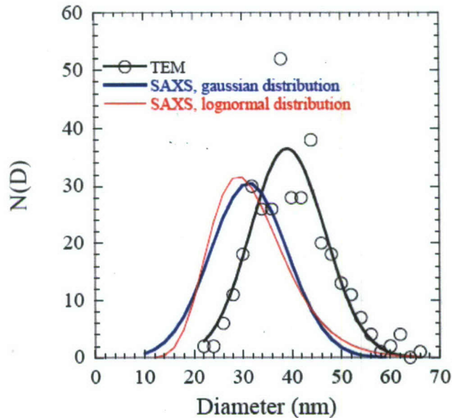
Figure 4 Comparison of size distributions obtained from a SAXS measurement and TEM images
