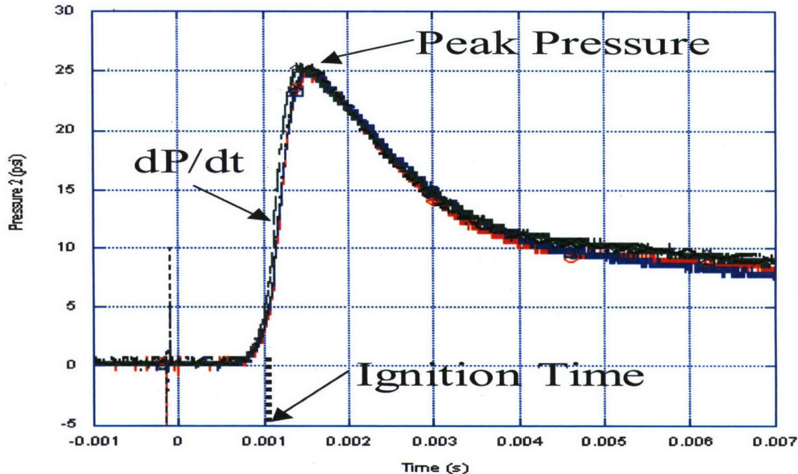
Figure 10 Pressure variations as a function of time indicate ignition time, peak pressure and pressurization rate
