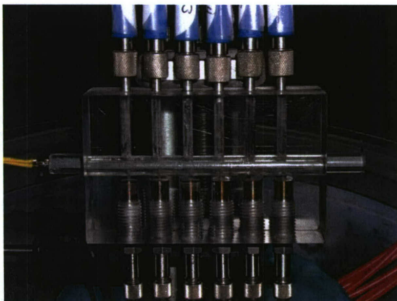
Figure 5 Instrumented burn tube test setup
