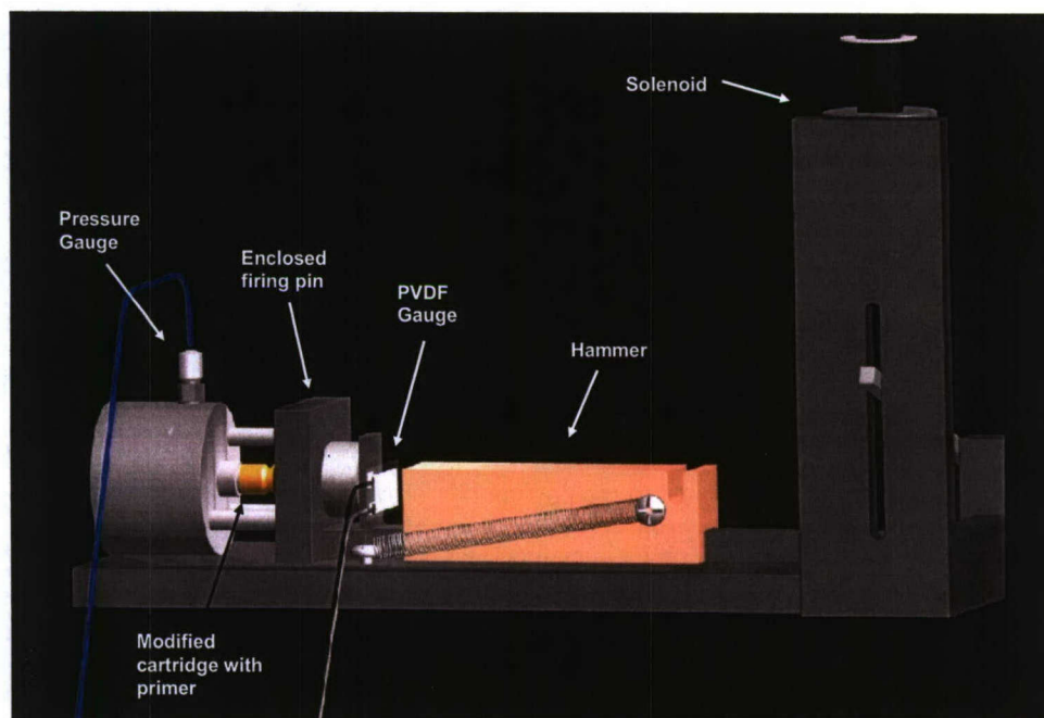
Figure 15 LANL primer firing pressure cell and firing mechanism computer model
