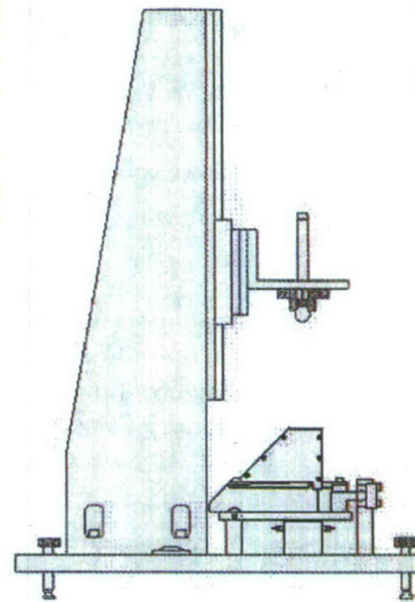
Figure 17 ARDEC primer drop test apparatus
