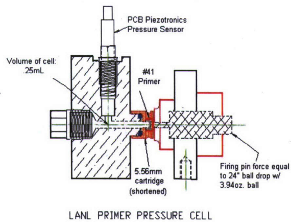
Figure 13 LANL primer firing pressure cell schematic
