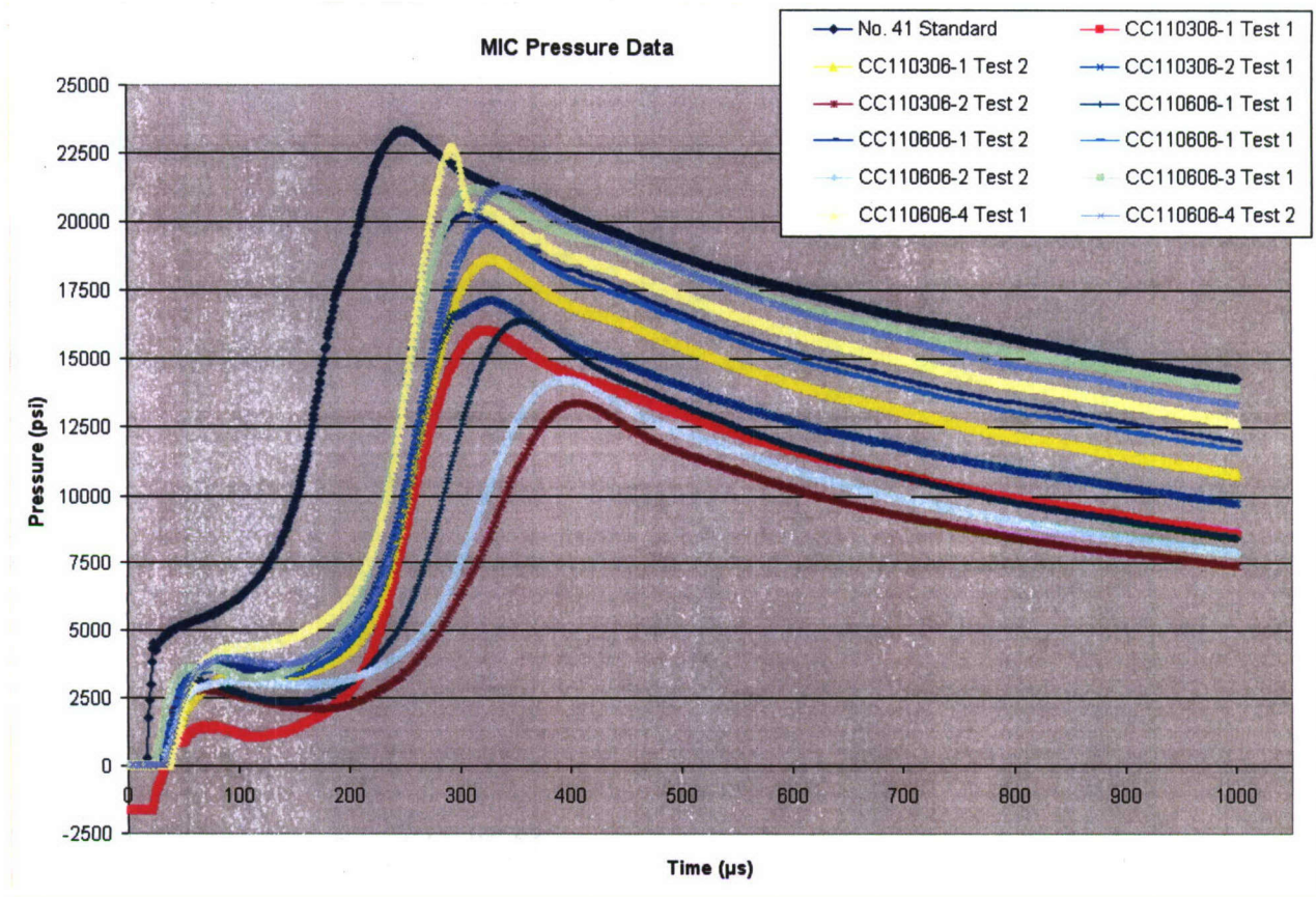
Figure 20 MIC primer laboratory P-t performance of final primer build
