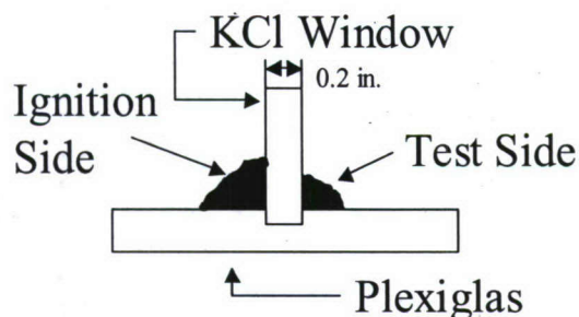
Figure 8 Radiant propagation setup
