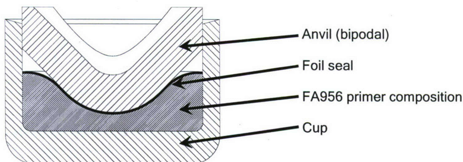
Figure 1 Cross-sectional sketch of the M115 percussion primer
