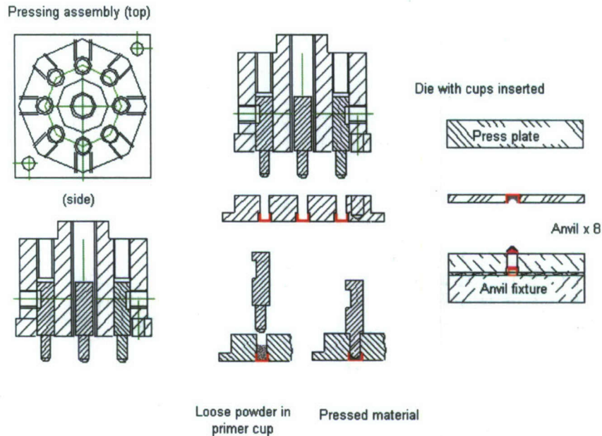
Figure 19 LANL primer press assembly for preparing experimental MIC No. 41 primers
