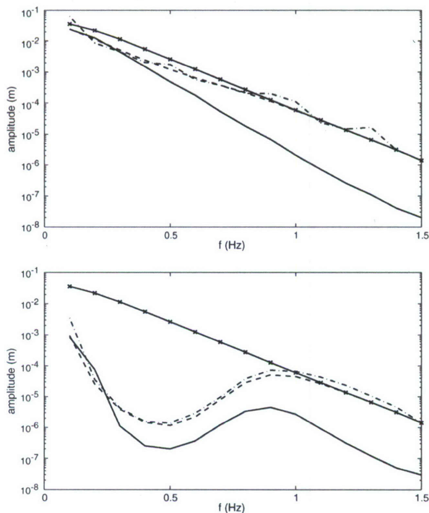
Fig. 7. One-dimensional cnoidal waves over mud patch with \gamma=0.9 : amplitudes of wavefield at x=0 (dash-x line) and at downwave end of mud patch ( x=800 m). Solid line: Eq. (11). Dashed line: Linear model. Dash-dot line: Eq. (11) with only superharmonic interactions. Top: \zeta=10 . Bottom: \zeta=100 .
