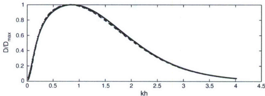
Fig. 2. Dissipation D (normalized by the maximum) as a function of relative water depth kh . Water depth h=1 m. Solid line: \zeta=10 , \gamma=0.9 , d_m=0.02 m. Dashed line: \zeta=100 , \gamma=0.9 , d_m=0.2 m. Dotted line: \zeta=10 , \gamma=0.5 , d_m=0.02 m. Dash-dot line: \zeta=100 , \gamma=0.5 , d_m=0.2 m.
