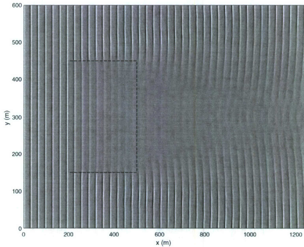
Fig. 8. Cnoidal waves propagating over two-dimensional mud patch: overhead view of free surface elevation (crests are in light streaks). Mud patch boundary shown in dashed lines. Mud parameters: d_m = 0.2 m, \gamma = 0.9 , \zeta = 100 .
