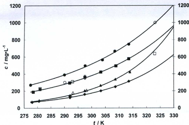
Figure 1. Solubility in pure water: \square , NT, ref 15; \blacksquare , NT, this study; \Delta , 2,6-DNT, ref 14 and 17; \blacktriangle , 2,6-DNT, this study; \circ , TNB, ref 16; \bullet , TNB, this study; \diamond , 2,3-DNT, ref 18; \blacklozenge , 2,3-DNT, this study. Error bars show the standard deviation of the concentration of replicate vials. Error bars for temperature are not included.
