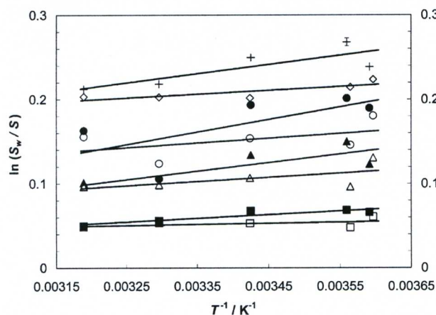
Figure 2. van't Hoff plot of NT and 2,3-DNT in seawater at various concentrations: \square , NT, 25 % seawater; \Delta , NT, 50 % seawater; \circ , NT, 75 % seawater; \diamond , NT, 100 % seawater; \blacksquare , 2,3-DNT, 25 % seawater; \blacktriangle , 2,3-DNT, 50 % seawater; \bullet , 2,3-DNT, 75 % seawater; + , 2,3-DNT, 100 % seawater.
