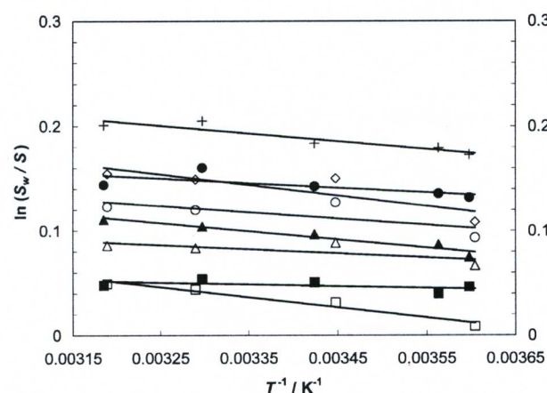
Figure 3. van't Hoff plot of TNB and 2,6-DNT in seawater at various concentrations: \square , TNB, 25 % seawater; \Delta , TNB, 50 % seawater; \circ , TNB, 75 % seawater; \diamond , TNB, 100 % seawater; \blacksquare , 2,6-DNT, 25 % seawater; \blacktriangle , 2,6-DNT, 50 % seawater; \bullet , 2,6-DNT, 75 % seawater; + , 2,6-DNT, 100 % seawater.
