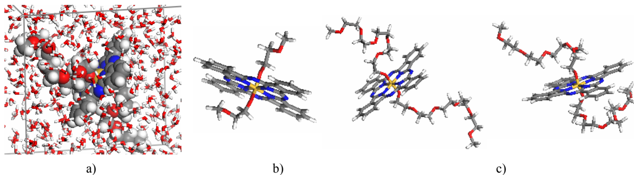
Figure 2. a) Unit cell of SiPC-PEG 250 with 500 water molecules. Conformers of b) SiPC-PEG 75 and c) SiPC-PEG 250
