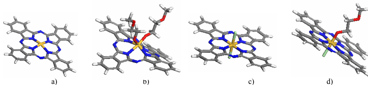
Figure 3. Conformers of SiPC with PEG 75 and Cl.
