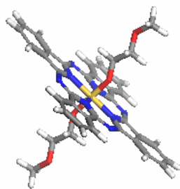
Figure 1. Structure of SiPC-PEG 75
