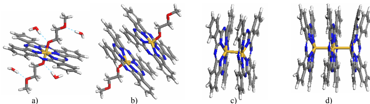
Figure 4. Structure of SiPC-PEG 75 with hydrogen-bonded water molecules and complexes of stacked SiPC fragments.
