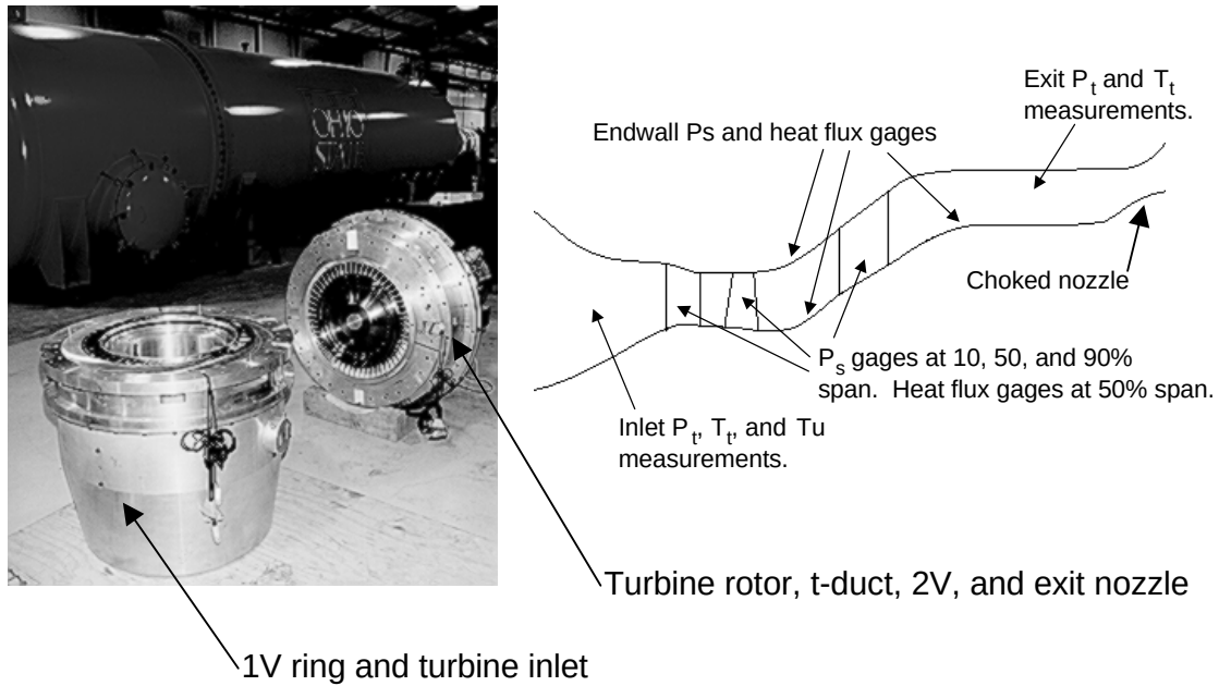
Fig. 3.1 The 1+1/2 stage transonic turbine tested at OSU for this study was heavily instrumented on airfoils in each row and along the rig flowpath.
