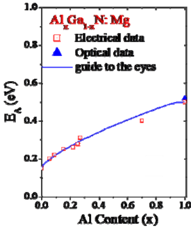
Fig. 5 Mg acceptor energy level in Al_xGa_{1-x}N alloys as a function of x .
